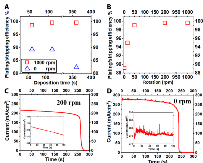
Fig. 6. Electrochemical reversibility of Zn electrodeposits measured in a 2.5 M \text{ZnSO}_4 (aq) electrolyte. (A) Coulombic efficiency for Zn plating/stripping with and without rotation. (B) Coulombic efficiency for Zn plating/stripping at different RDE rotation rates. Time-dependent evolution of the current density during stripping of Zn deposited (C) with and (D) without normal flow.
